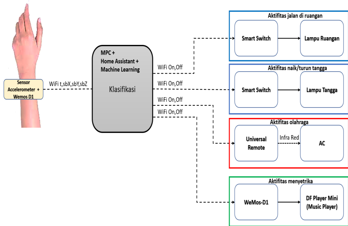
Figure 2. Block Diagram System Introduction To Activity Movement.
