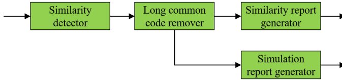
Fig. 2. Overview of similarity feedback generator.
