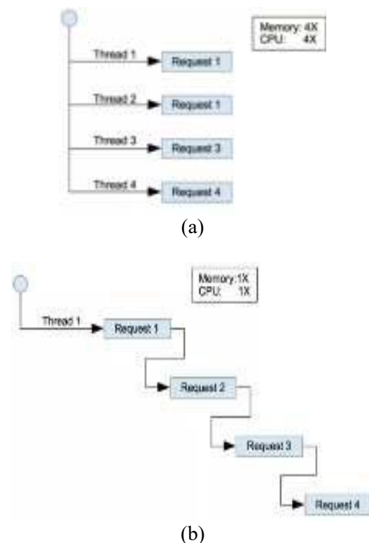
Gambar 5. Analogi Pemrosesan (a) multi threaded (b) single threaded
