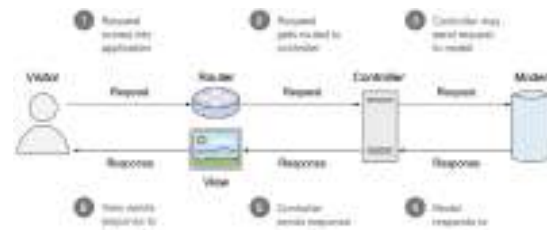
Gambar 2. Alur web framework
