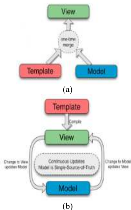
Gambar 4. (a) One-way dan (b) Two-way Data Binding
